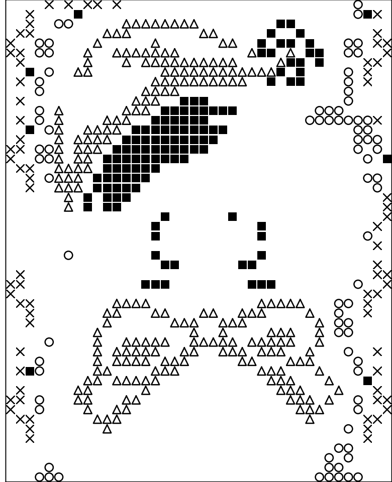
Plaque 1 100 = ■ 109 = ○ 114 = × 134 = △
