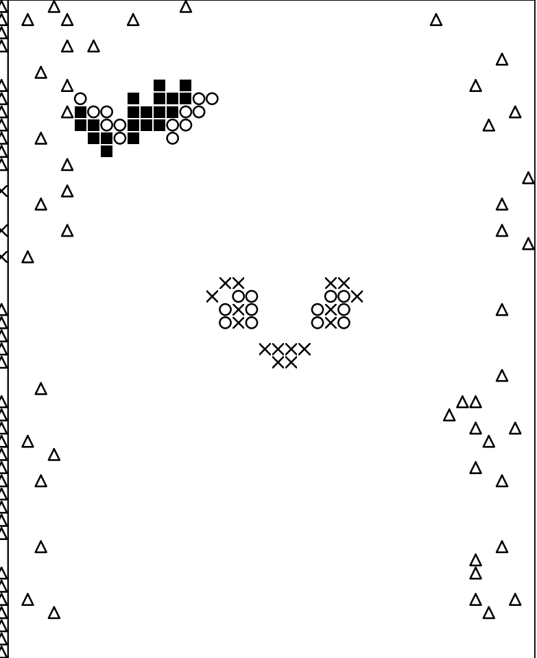
Plaque 1 341 = ■ 342 = ○ 441 = × 468 = △
