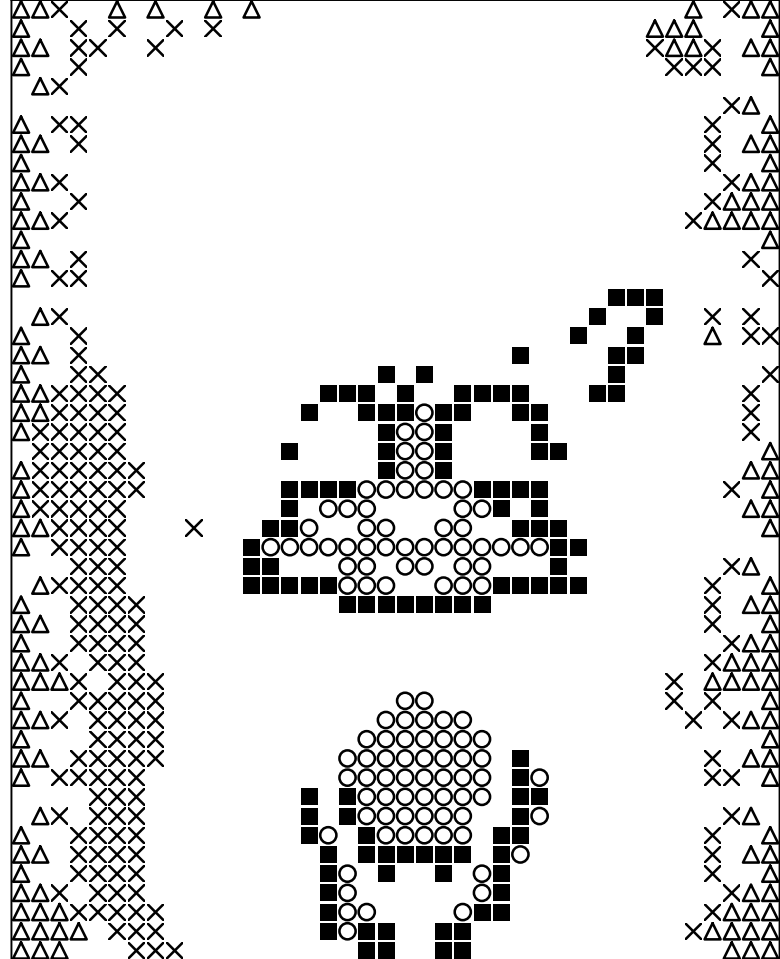
Plaque 1 257 = ■ 269 = ○ 288 = × 300 = △
