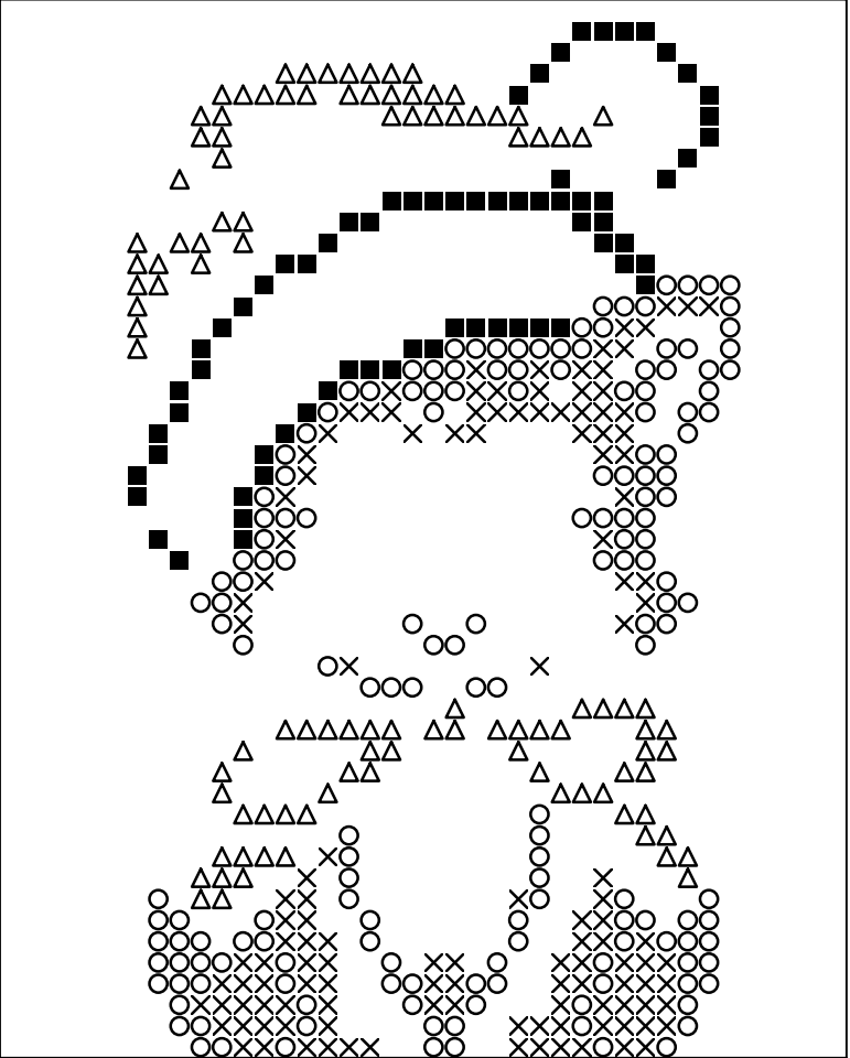
Plaque 1 173 = ■ 177 = ○ 178 = × 224 = △
